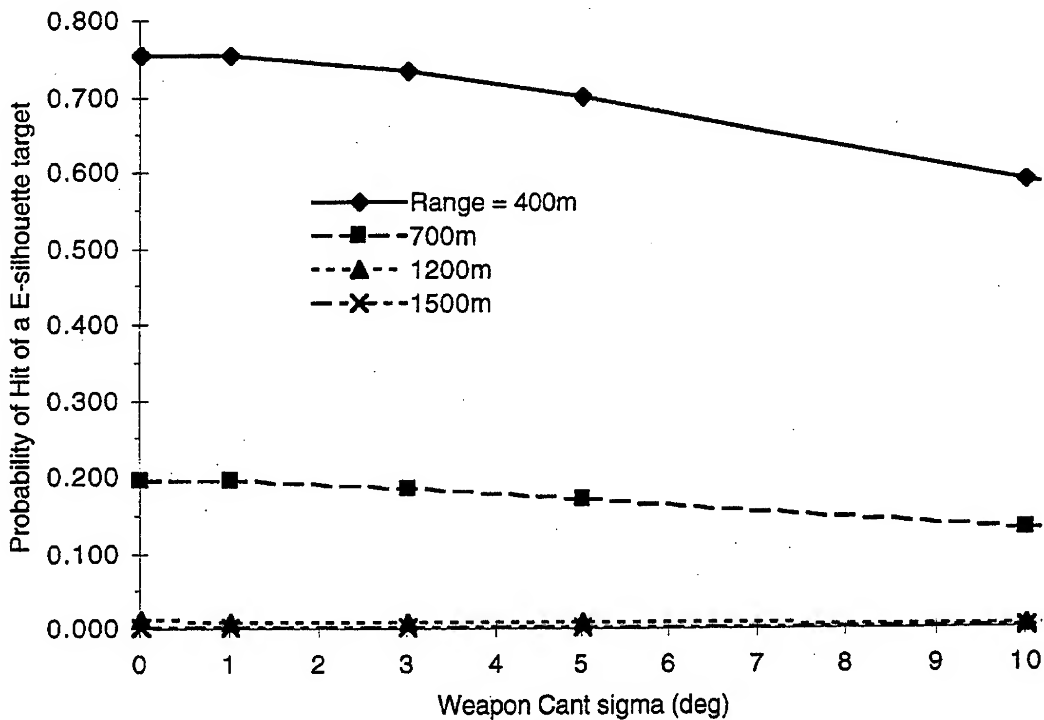
Figure D-2. Error Budget Sensitivity, Weapon Cant.
